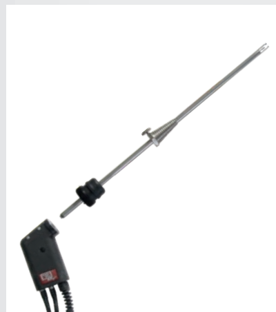
Large selection of probes and hoses for flue gas temperatures up to 1.100°C
