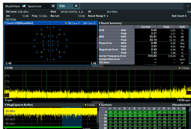
Demodulation of a DVB-SX2 multi-modulation signal with the R&S®FPL1-K70M option (R&S®FPL1-K70 option required)
