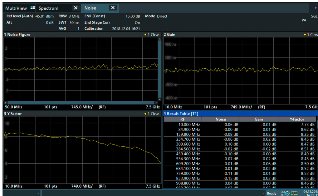
Simultaneous view of graphs for noise figure, gain and Y factor versus frequency and a table of the results in numerical format
