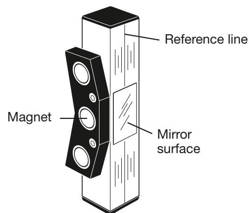
Reflector unit
